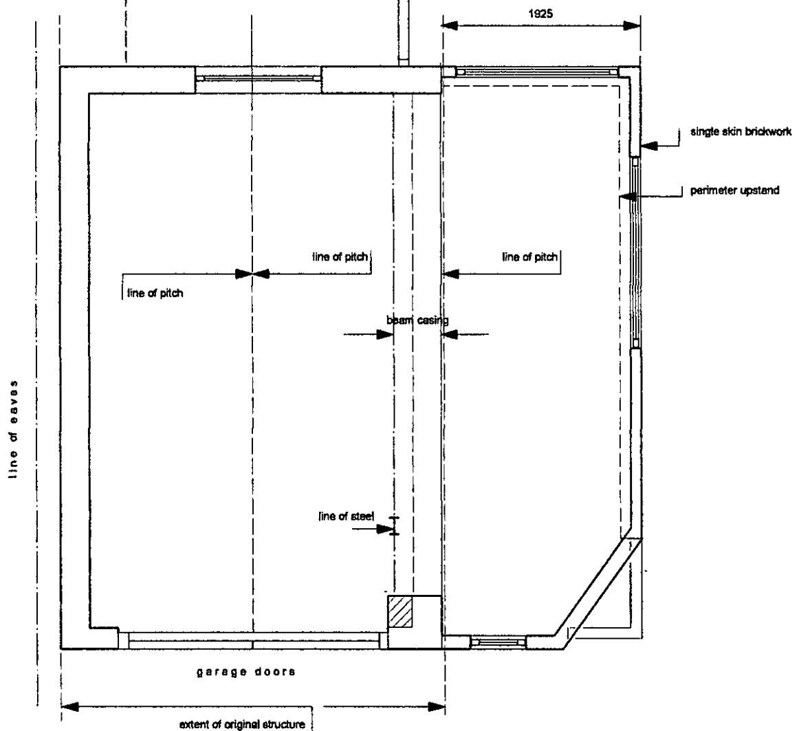
EXISTING PLAN
