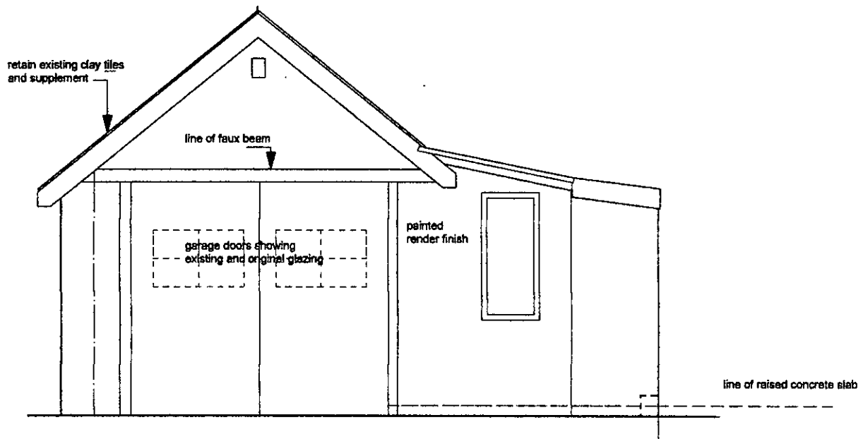
EXISTING WESTERN ELEVATION
