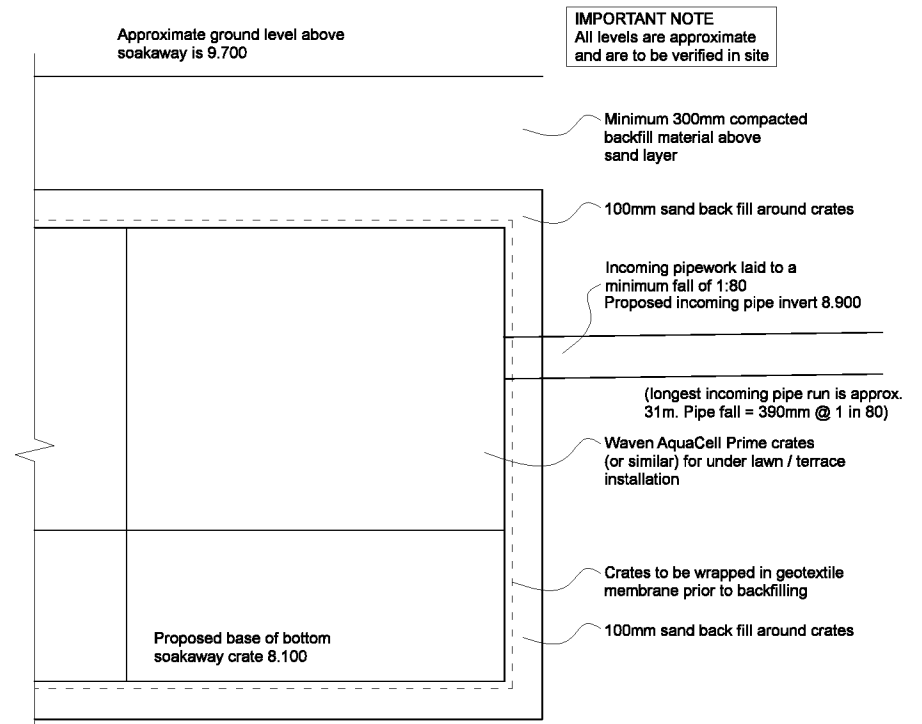
Rear Soakaway Detail SA02
