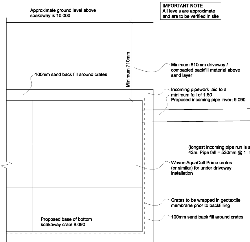
Front Soakaway Detail SA01
