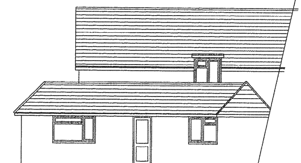
Existing West Elevation Conservatory not shown for clarity
