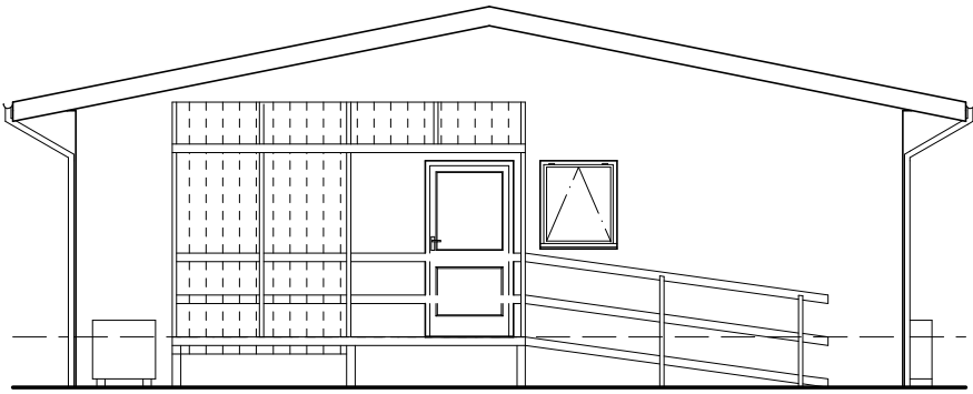
PROPOSED FRONT NORTH WEST FACING ELEVATION
