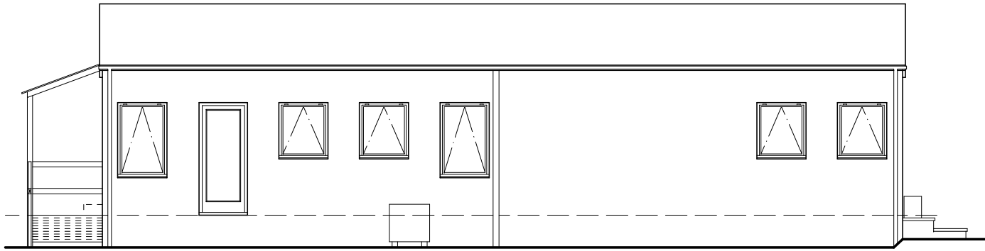
PROPOSED SIDE SOUTH WEST FACING ELEVATION
