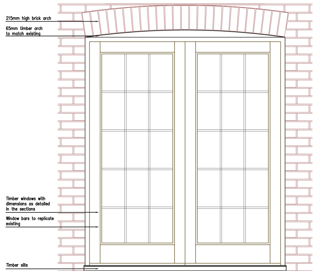
D1 1:20 French Doors Sliding folding doors have the same dimensions for door frames, stiles etc
