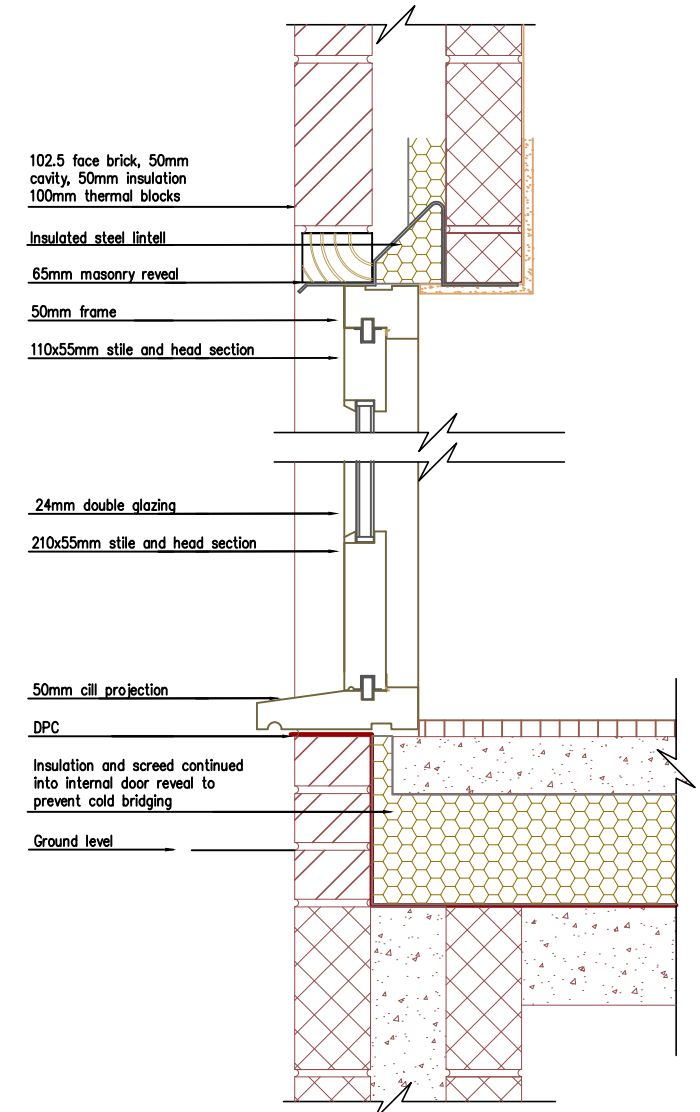
D3 1:10 SLiding Door Vertical Section
