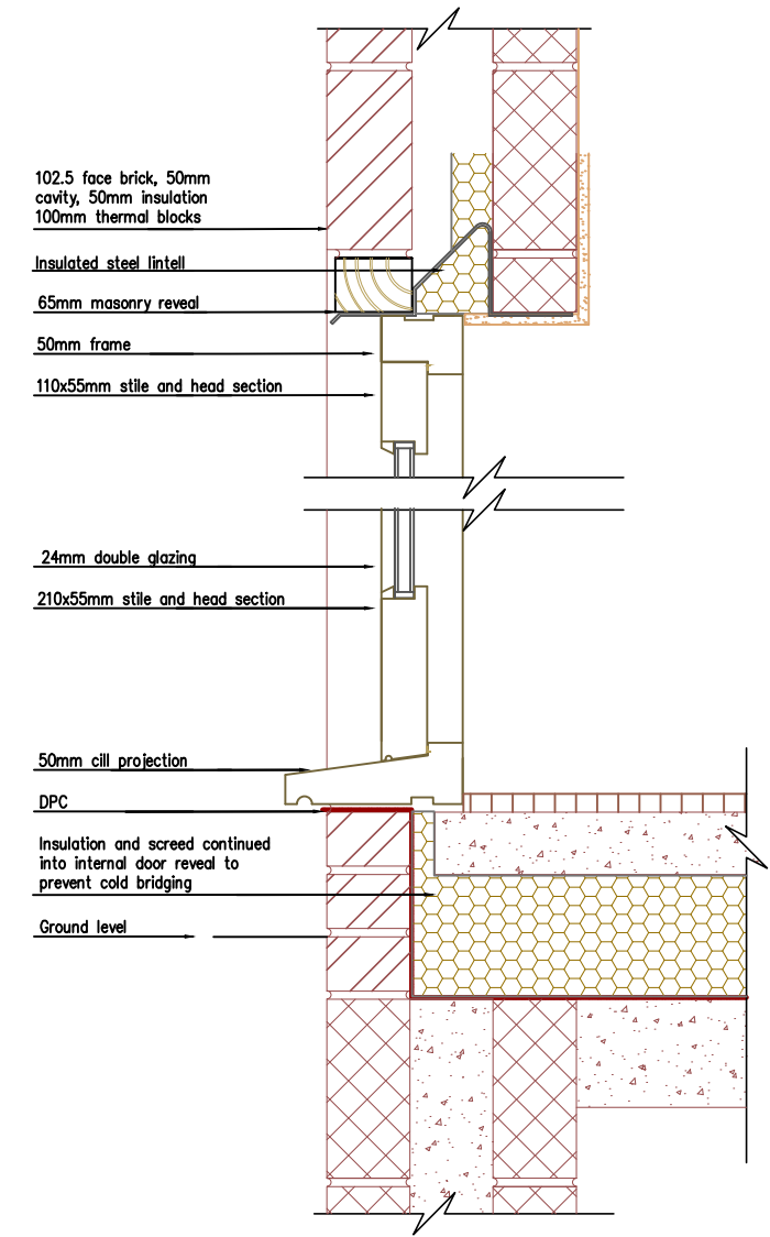
D4 1:10 French Door Vertical Section
