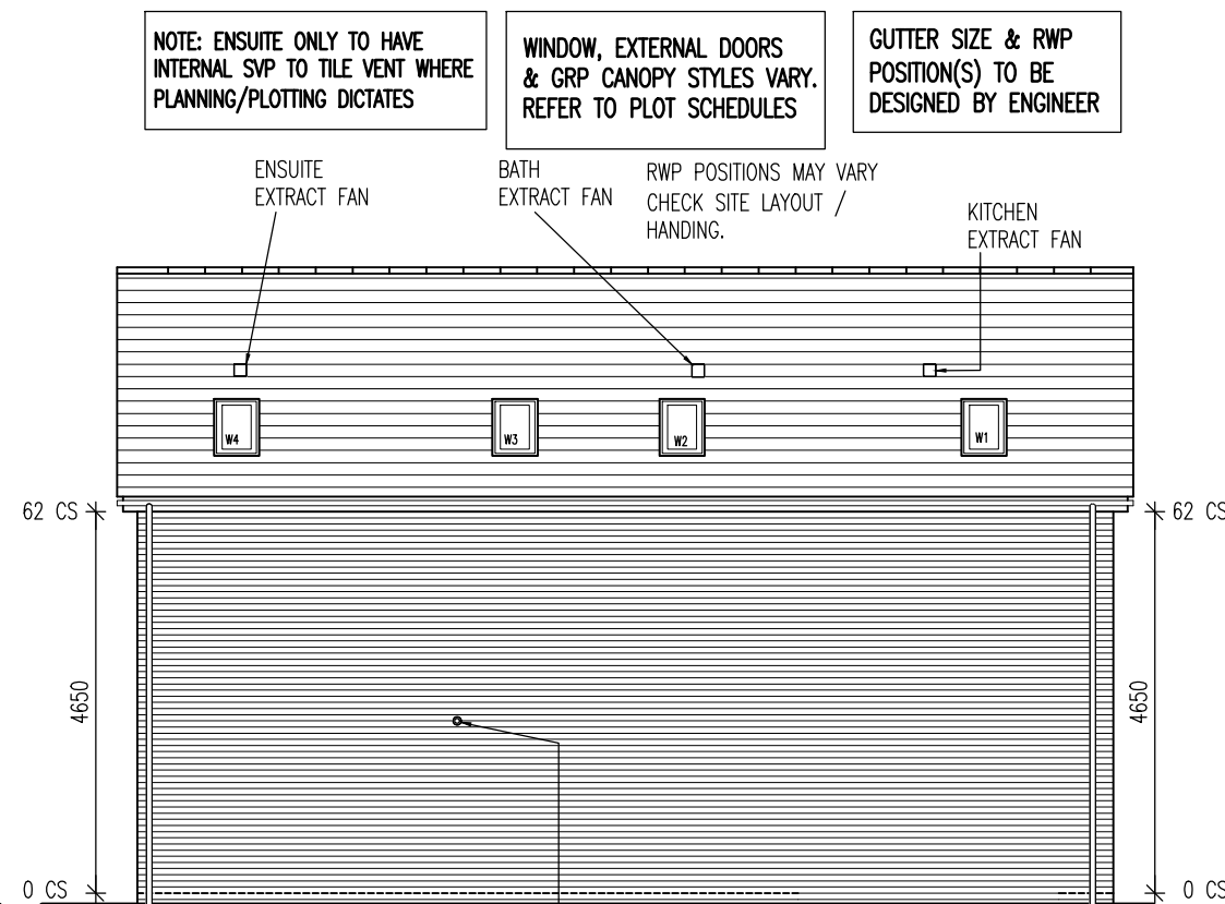
REAR ELEVATION
