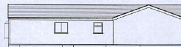
Elevation rear/south @ 1:100
