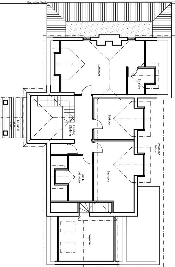
03 Proposed Upper Floor Plan 1:200
