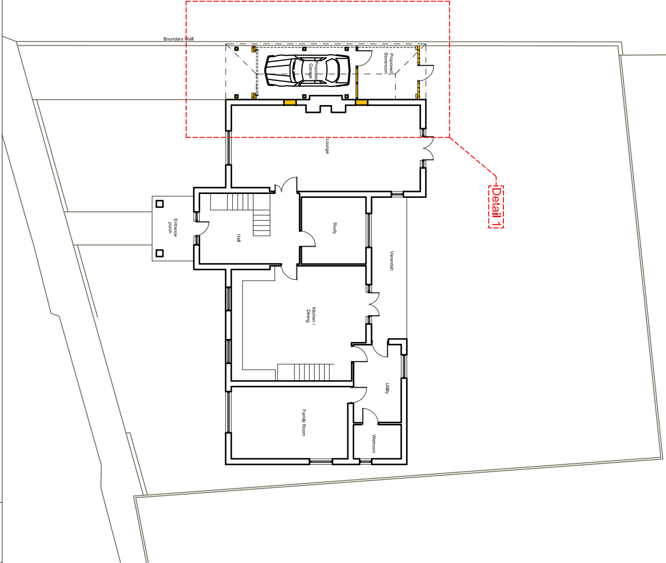
01 Proposed Ground Floor Plan 1:200
