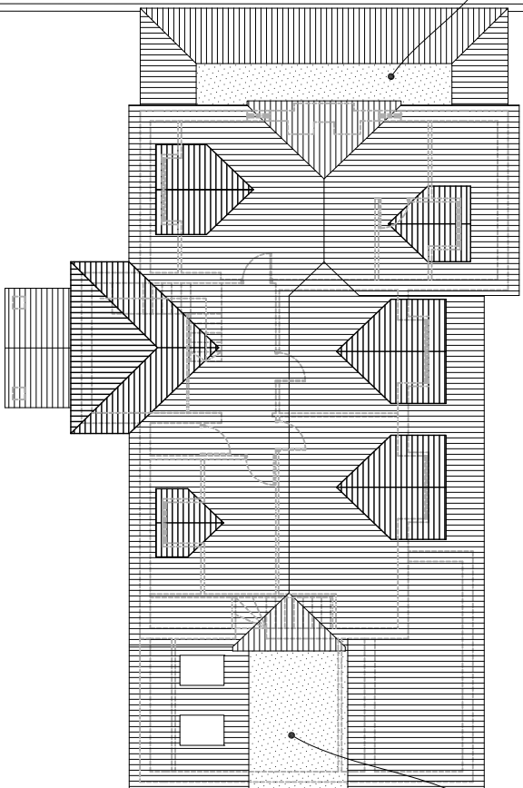
04 Proposed Roof Plan 1:200
