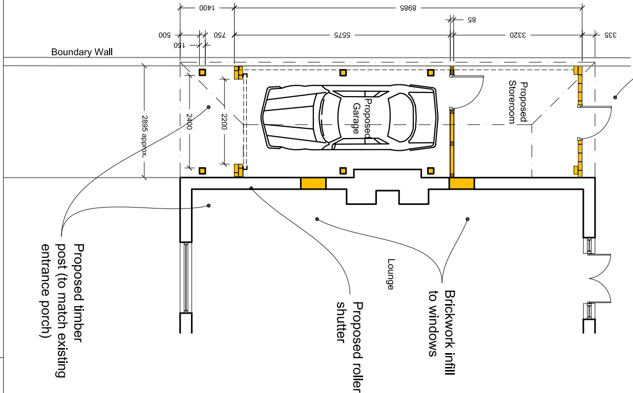
02 Detail 1: Proposed (part) Plan - Garage 1:100
