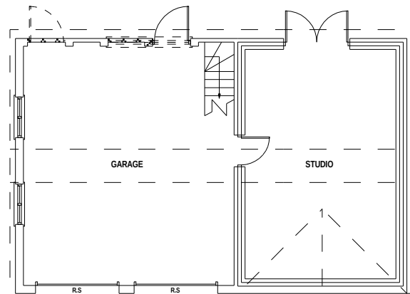
PROPOSED GROUND FLOOR LAYOUT SCALE 1:50
