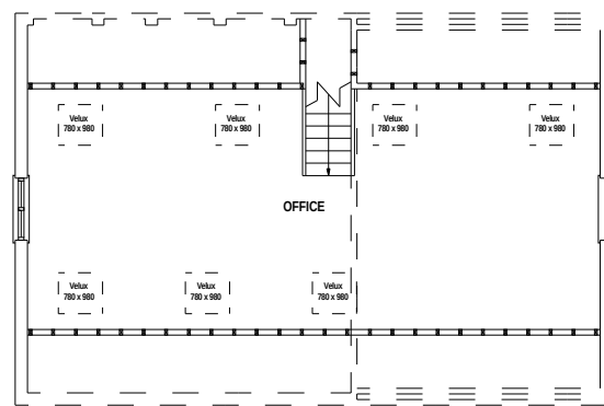
PROPOSED FIRST FLOOR LAYOUT SCALE 1:50
