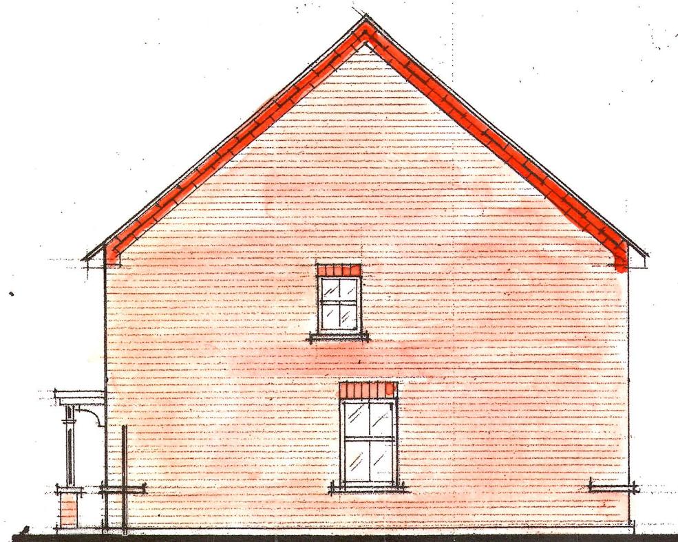
plot 2, 4 & 6 WEST ELEVATION
