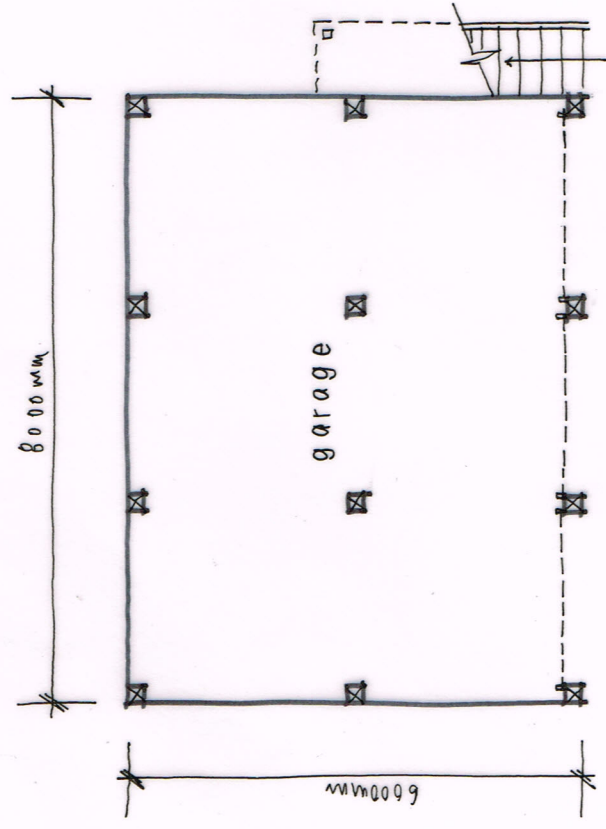
GROUND FLOOR PLAN 1:100 @ A3 / 1:50 @ A1
