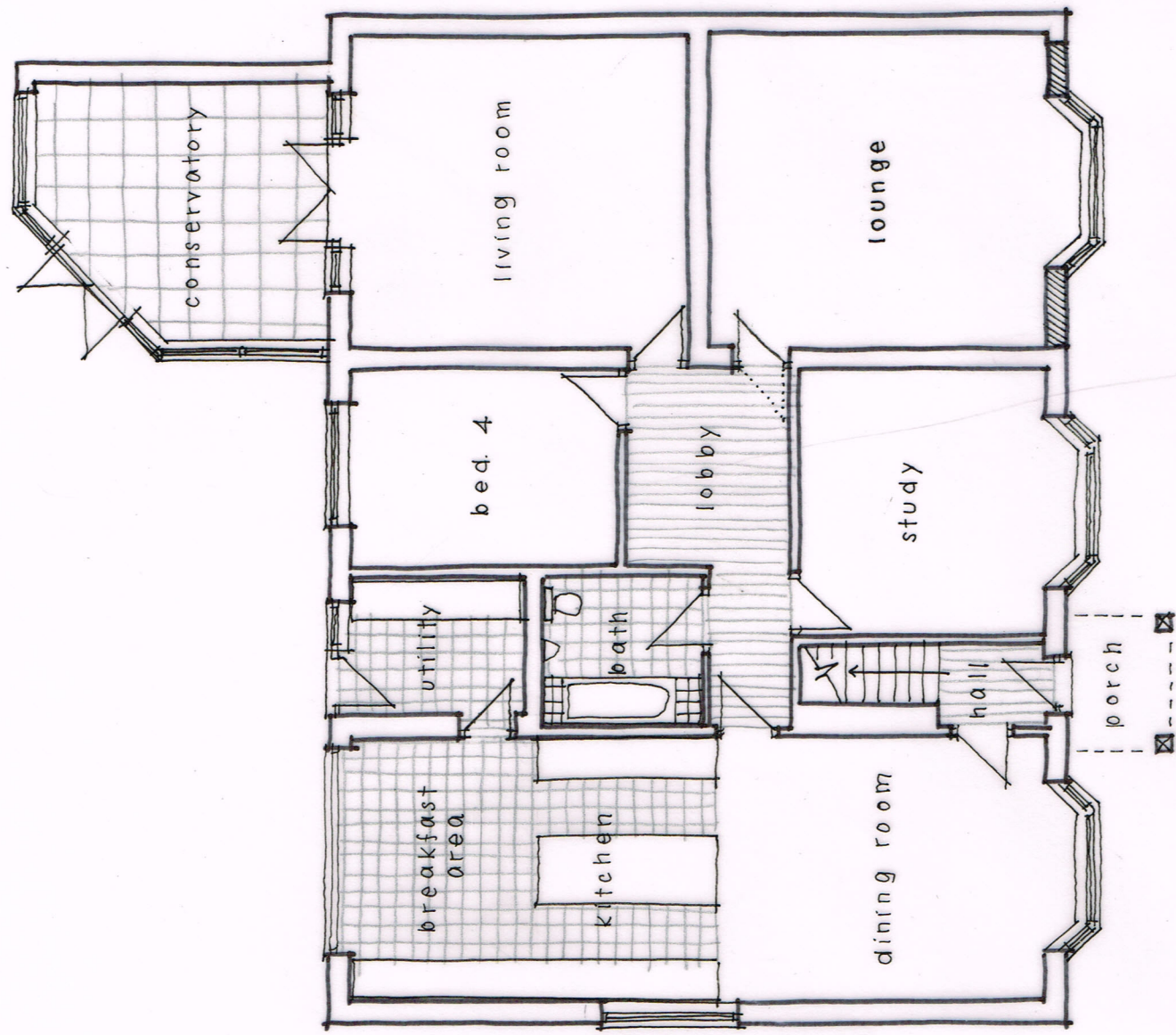
GROUND FLOOR PLAN 1:100 @ A3 / 1:50 @ A1
