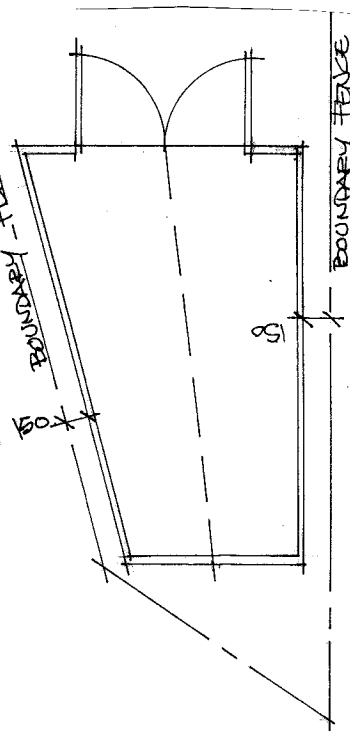
GARDEN SHED PLAN. 1:50
