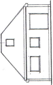
SOUTH ELEVATION
