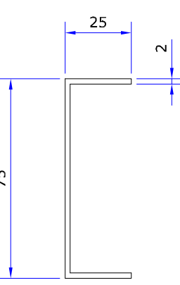
DETAIL 2 - SCALE 1:2
