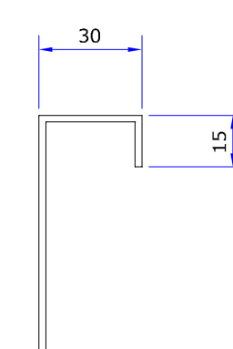
DETAIL 1 - SCALE 1:2
