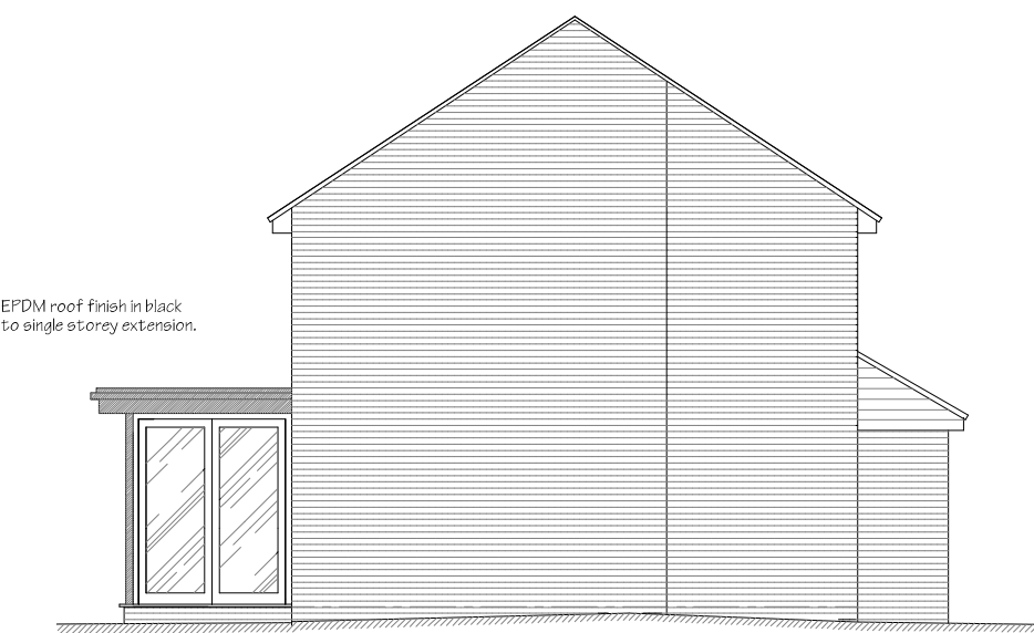
WEST ELEVATION (Side)
