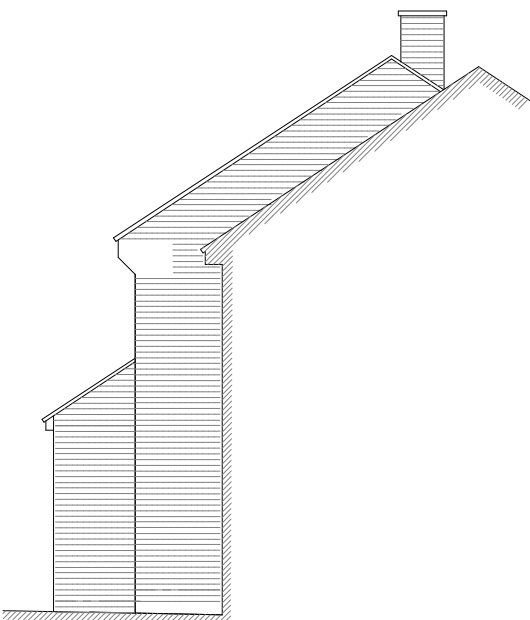
EAST ELEVATION (Side)
