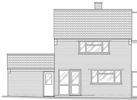
SOUTH ELEVATION (Front)
