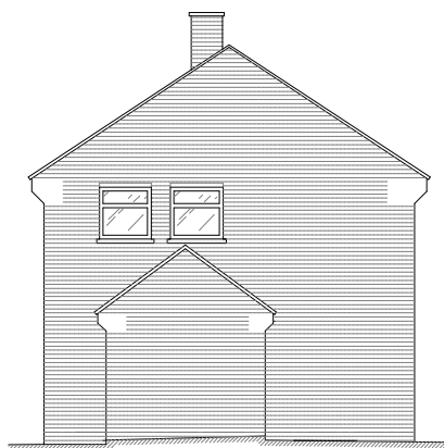
WEST ELEVATION (Side)
