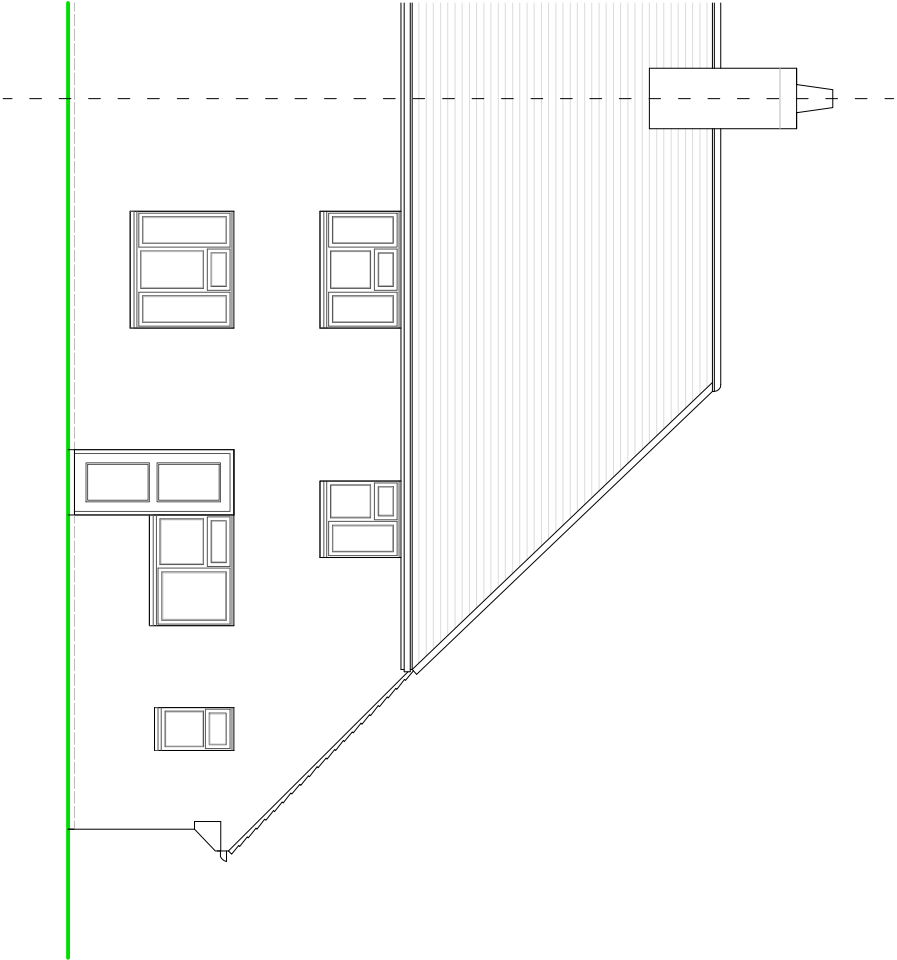
FRONT ELEVATION
