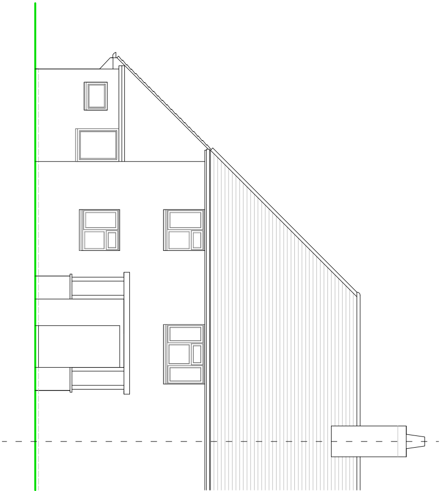
REAR ELEVATION
