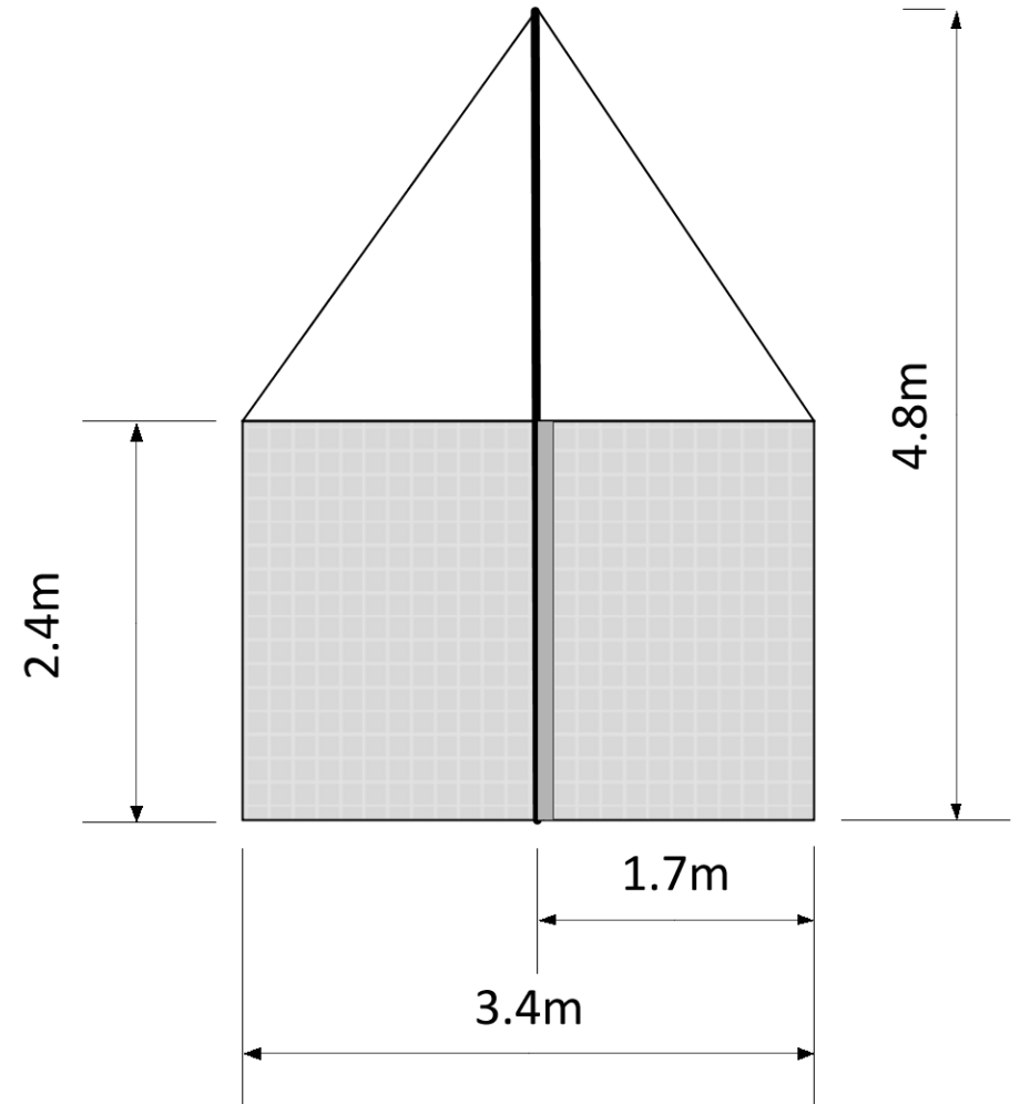
East Elevation
