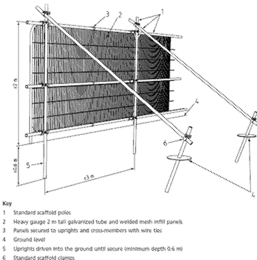
Figure 2: BS5837:2012 - Figure 2, Default specification for protective barriers.
