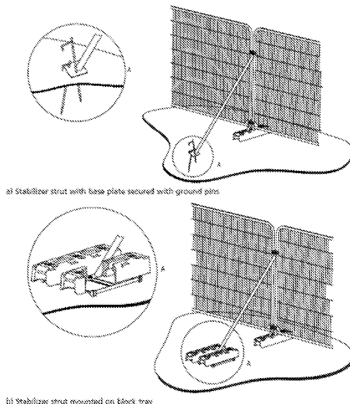
Figure 3: BS5837:2012 - Figure 3, Examples of above-ground stabilising systems.
