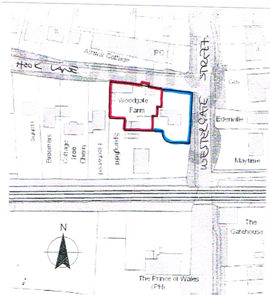
Location Plan (Extract from Ordnance Survey) Scale 1:1250
