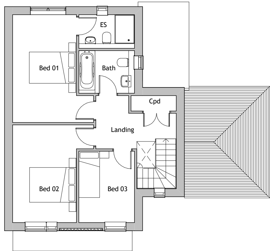
First Floor 1 : 100
