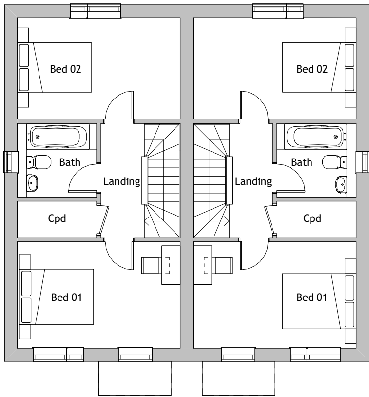
First Floor 1 : 100
