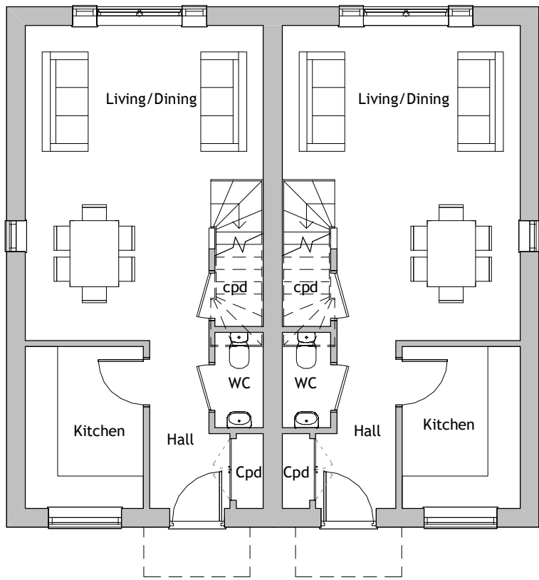
Ground Floor 1 : 100
