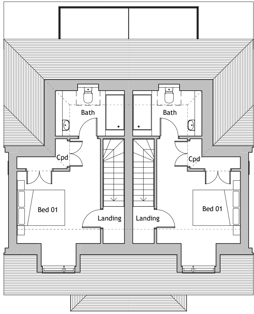
Second Floor 1 : 100
