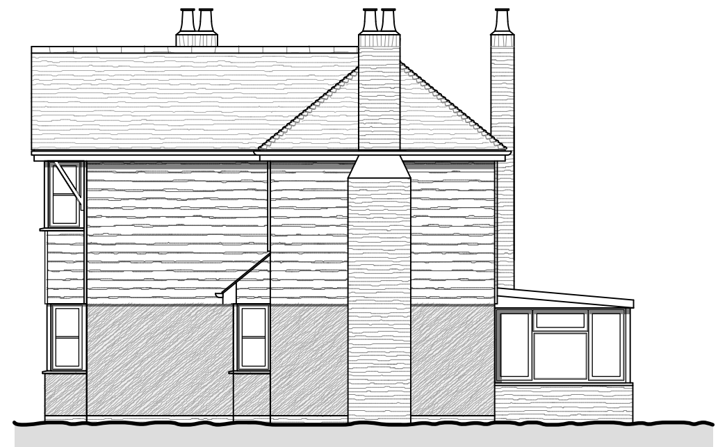
South-West Elevation
