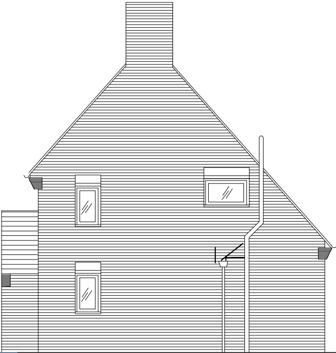
Existing East Elevation
