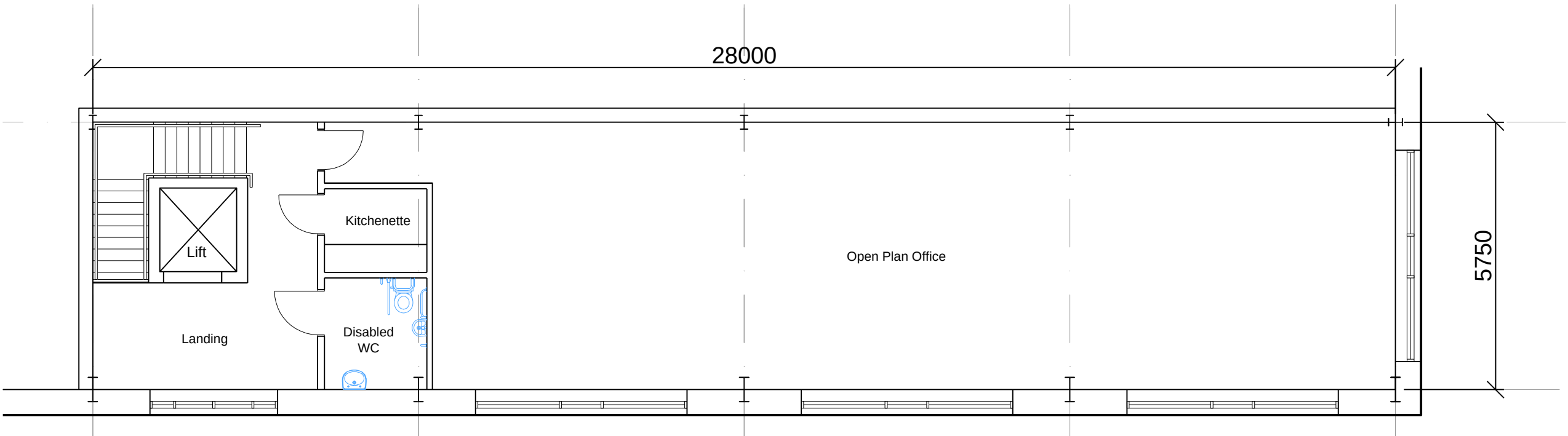
FIRST FLOOR OFFICE
