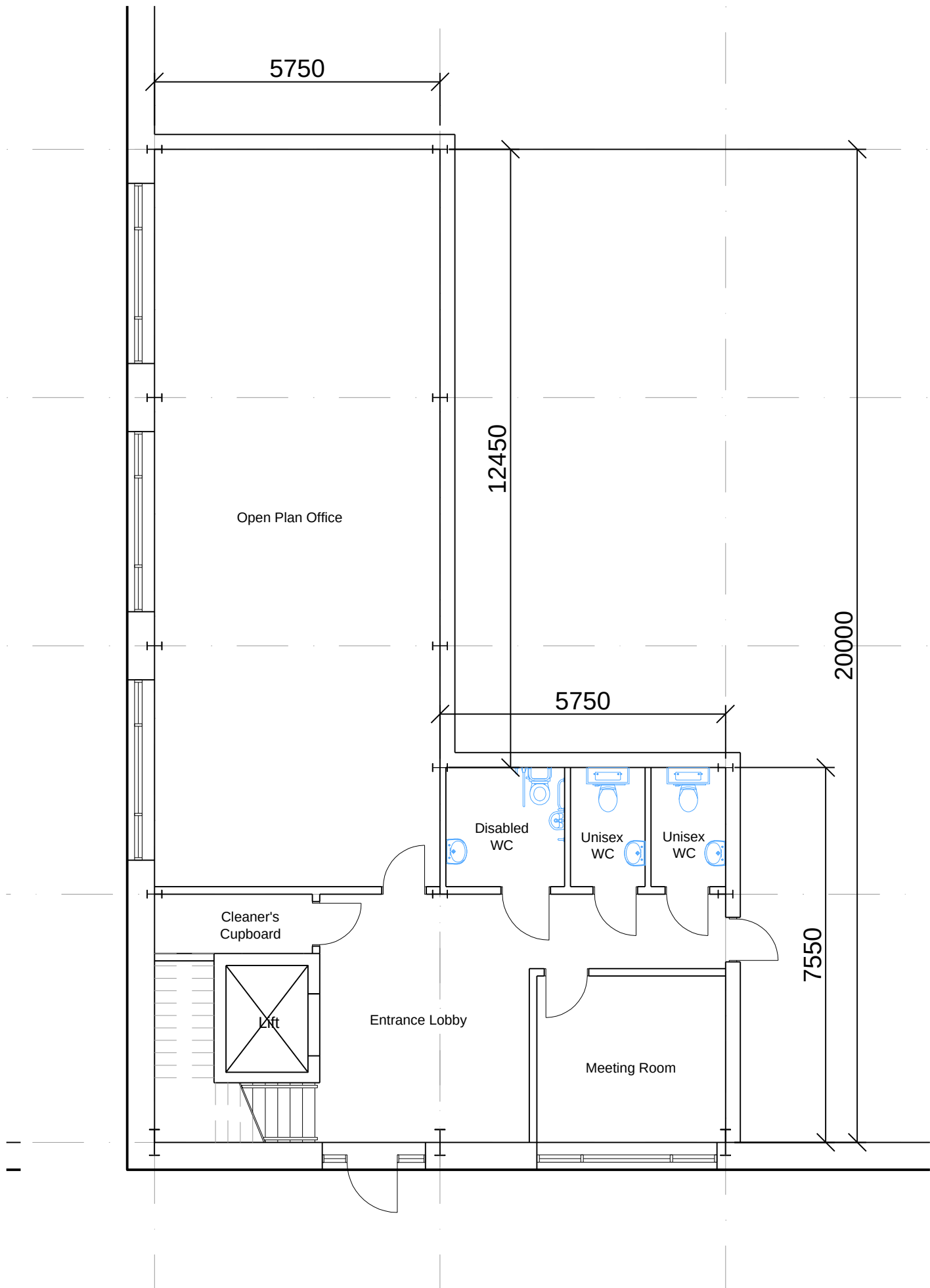
GROUND FLOOR OFFICE
