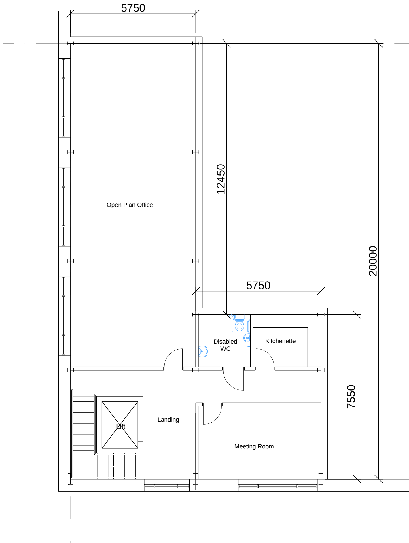
FIRST FLOOR OFFICE
