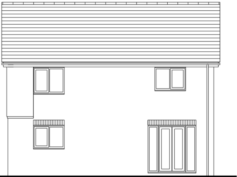
REAR ELEVATION
