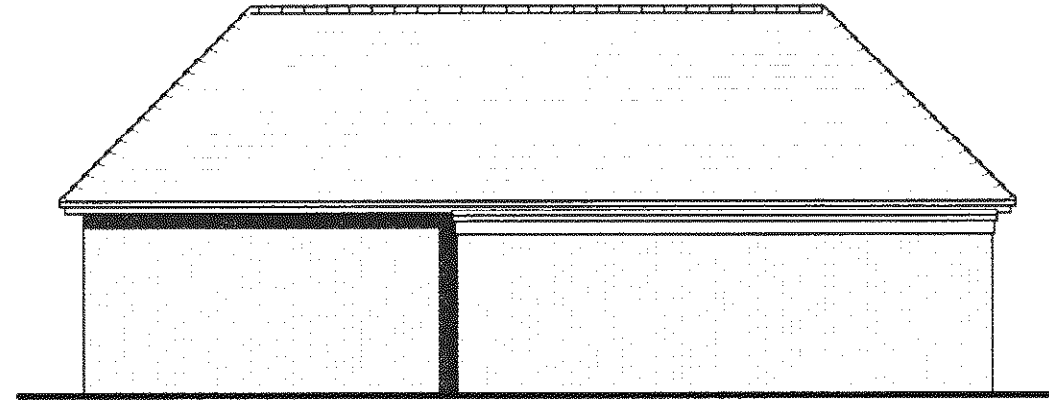
Proposed North Elevation Scale 1:100
