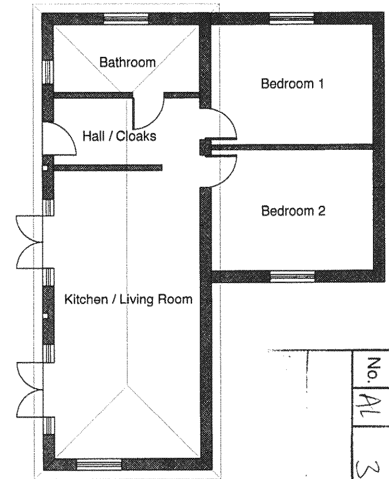
Proposed Floor Plan Scale 1:100
