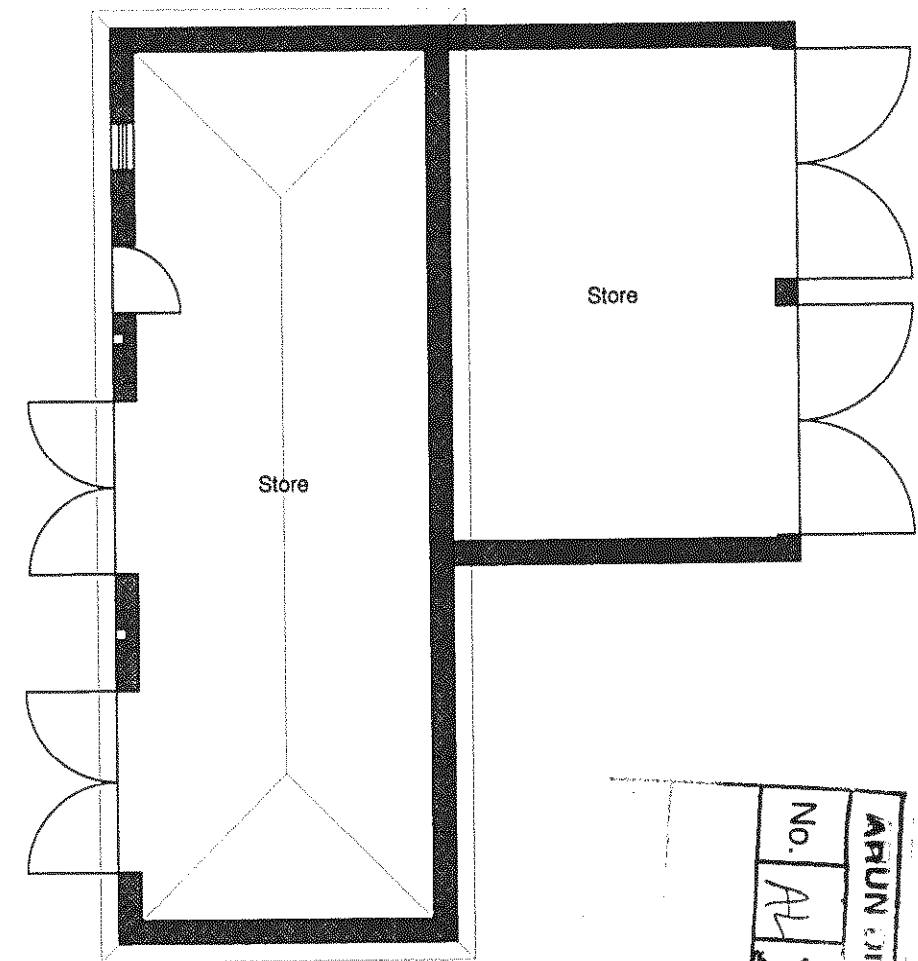
Existing Floor Plan Scale 1:100
