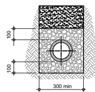
GRANULAR SURROUND (CLASS S)
