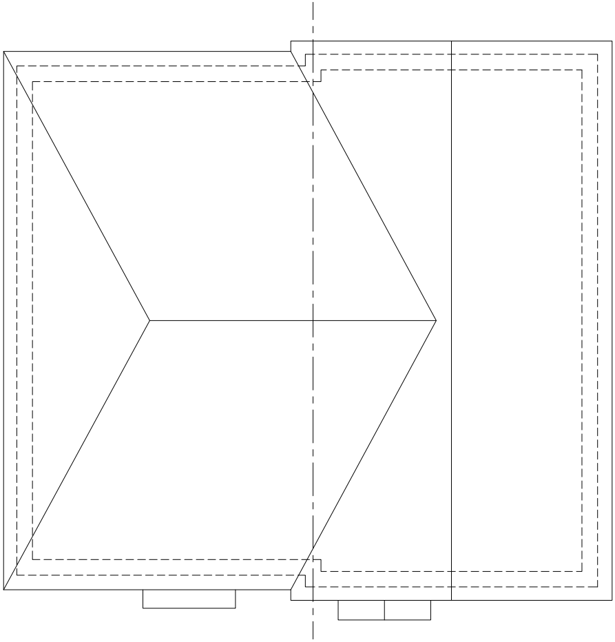
ROOF plan
