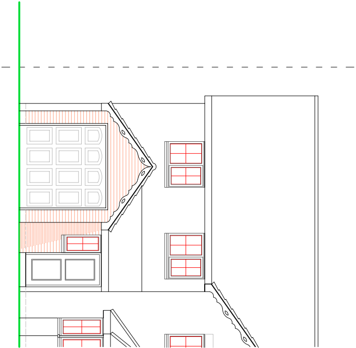
FRONT ELEVATION
