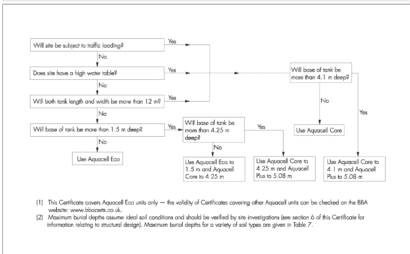
Figure 2 Sustainable drainage system selection and design
