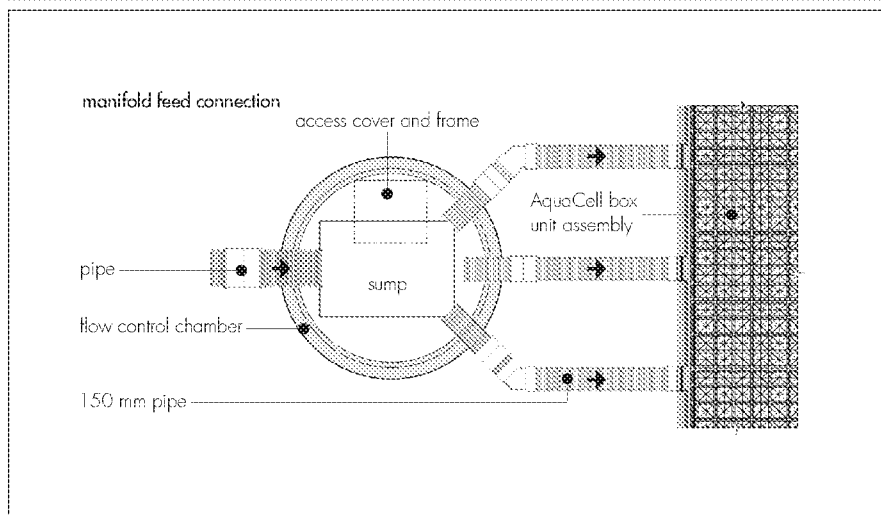
Figure 3 Typical inlet connection design
