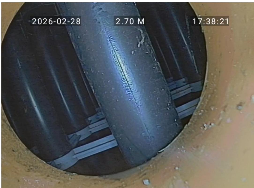
Finish node, soakaway, reference: SA35
