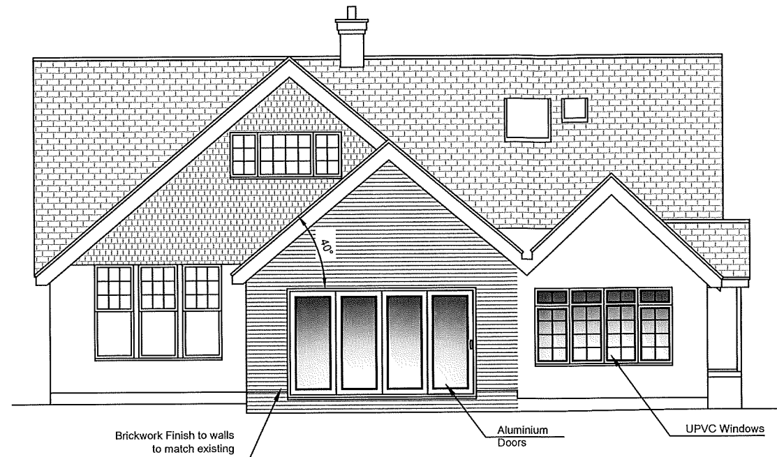
Rear Elevation
