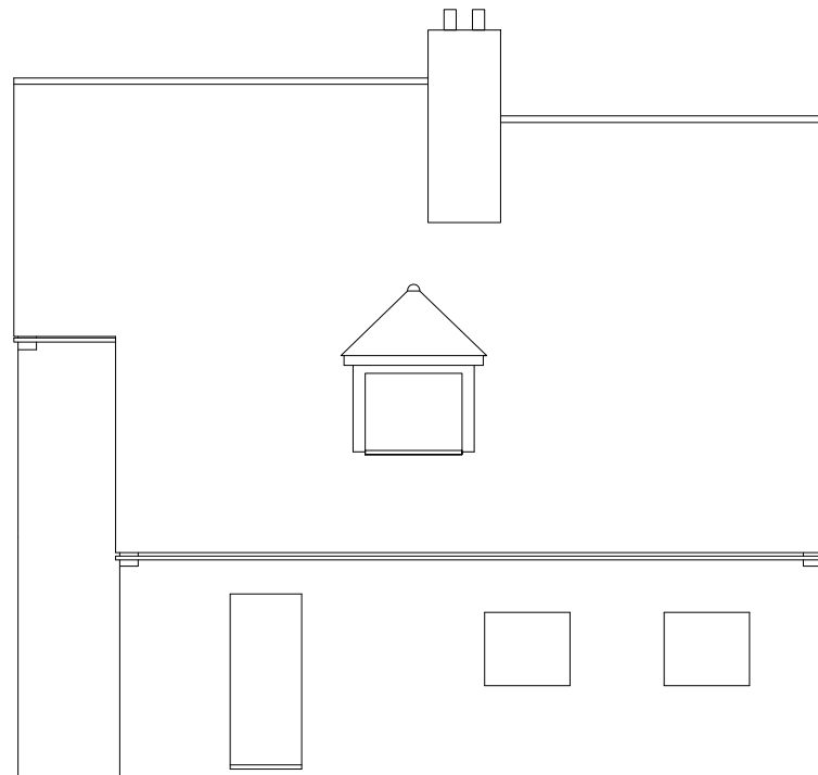
SIDE ELEVATION (NORTH)
