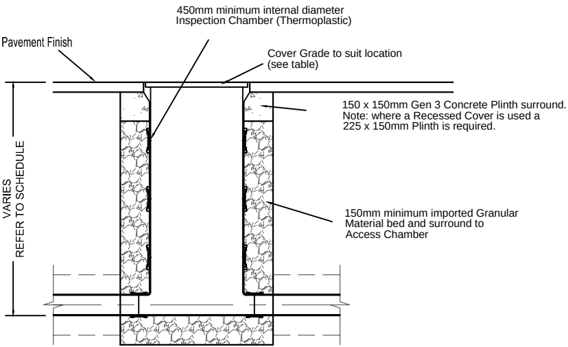
Typical Inspection Chamber
