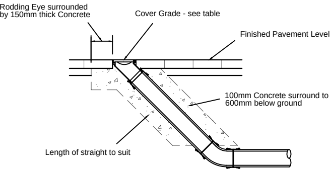
Typical Rodding Eye Access Point Detail
