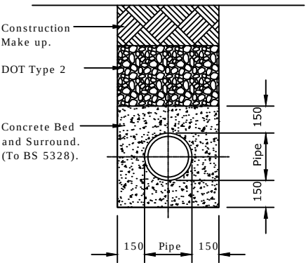
Typical Rainwater Pipe Connection Detail
