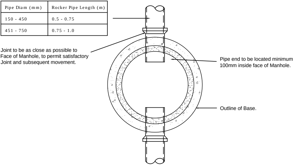
Typical Silt Trap Detail.
