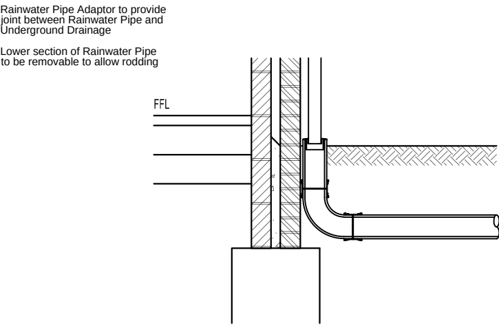
Typical Rainwater Pipe Connection Detail
