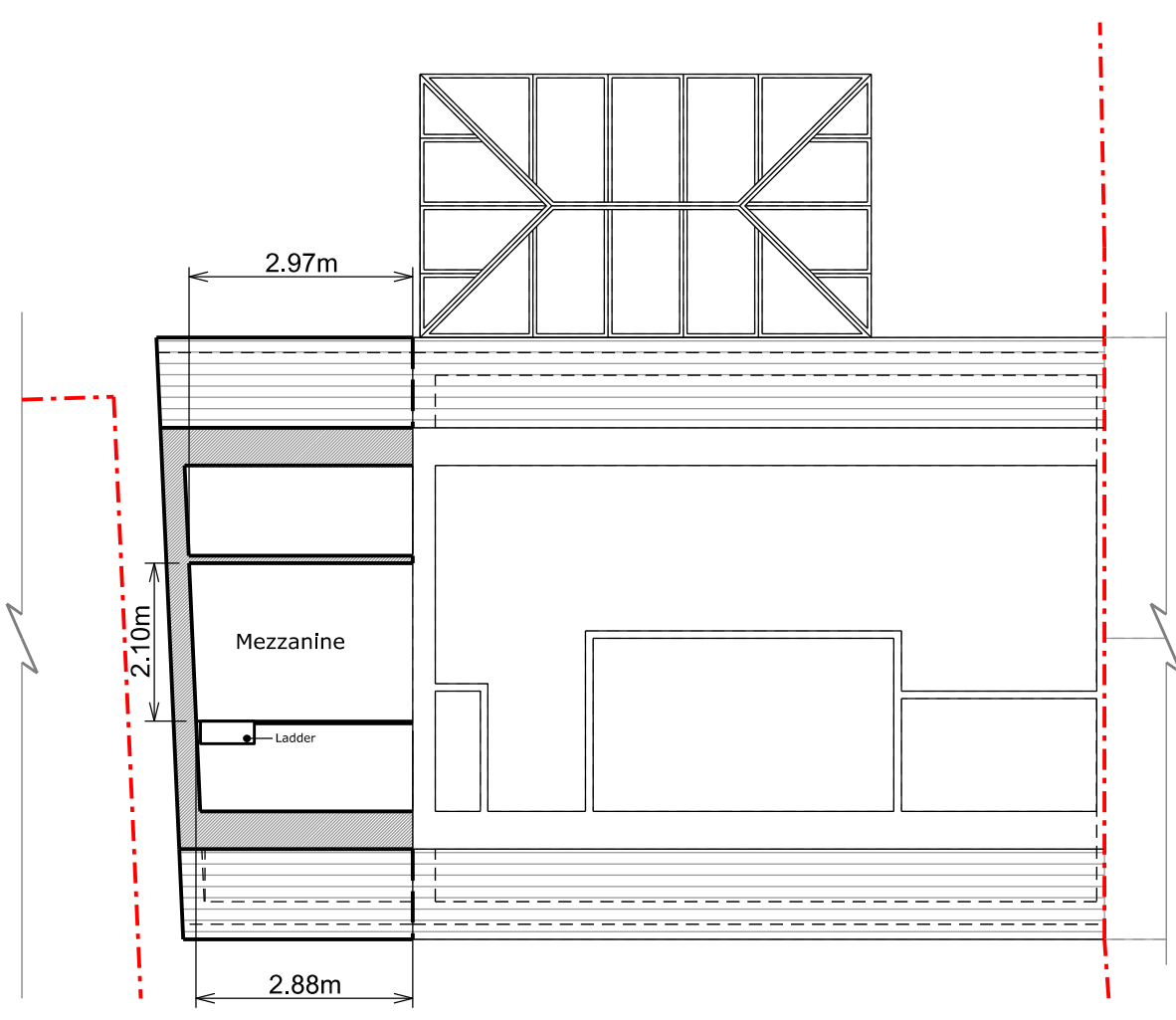
Mezzanine Floor Plan
