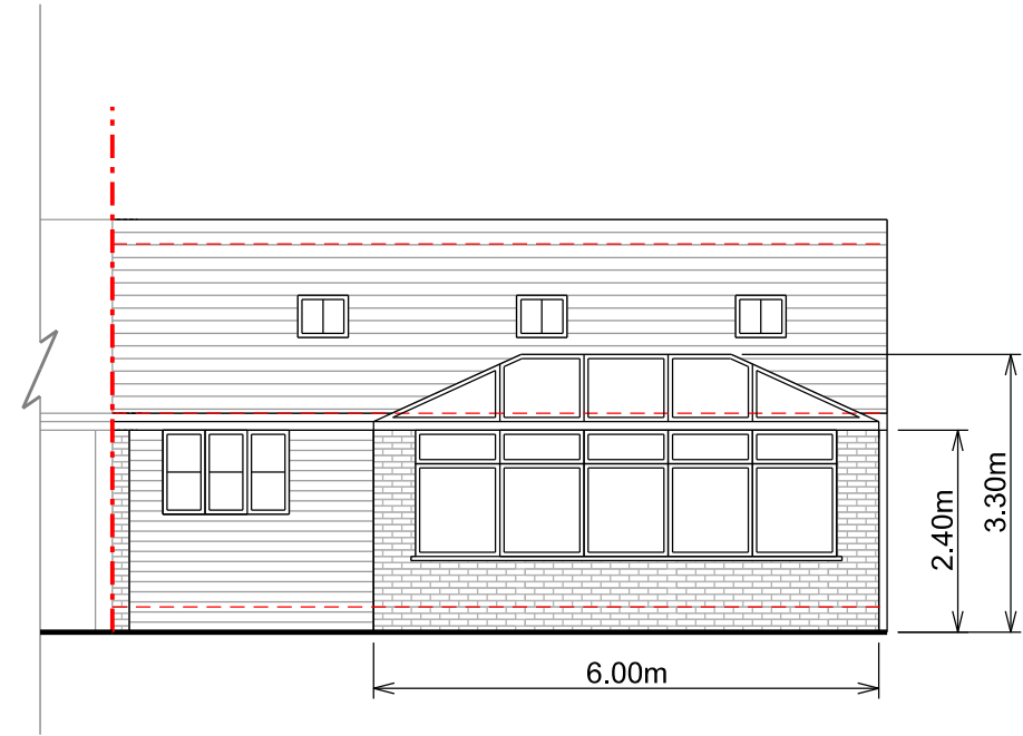
Rear Elevation
