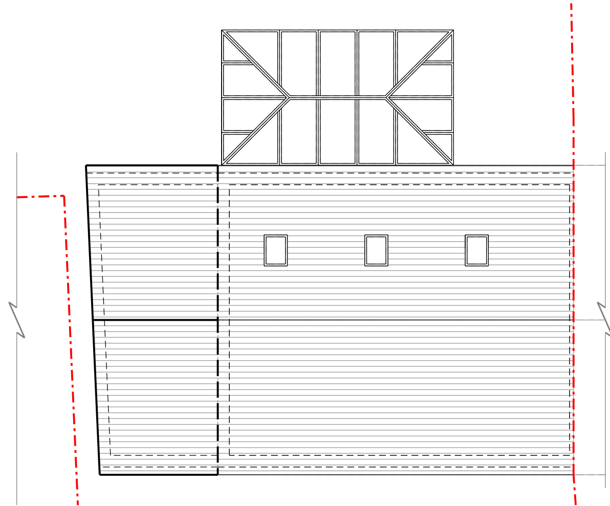
Roof Plan
