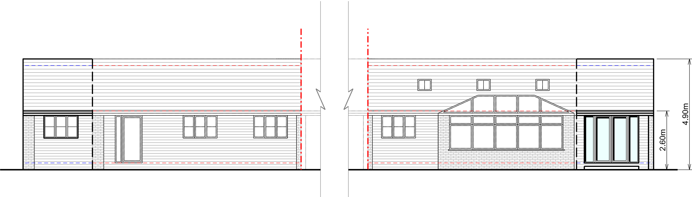
Front Elevation
