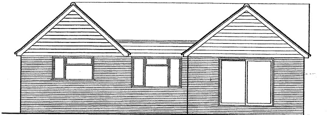
REAR ELEVATION
