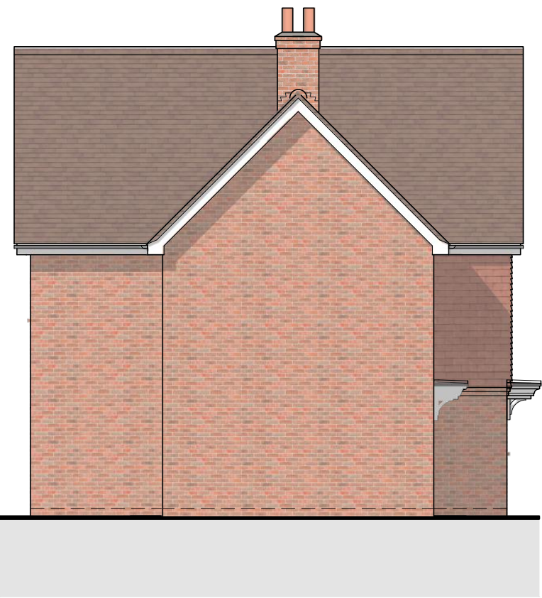
SIDE elevation
