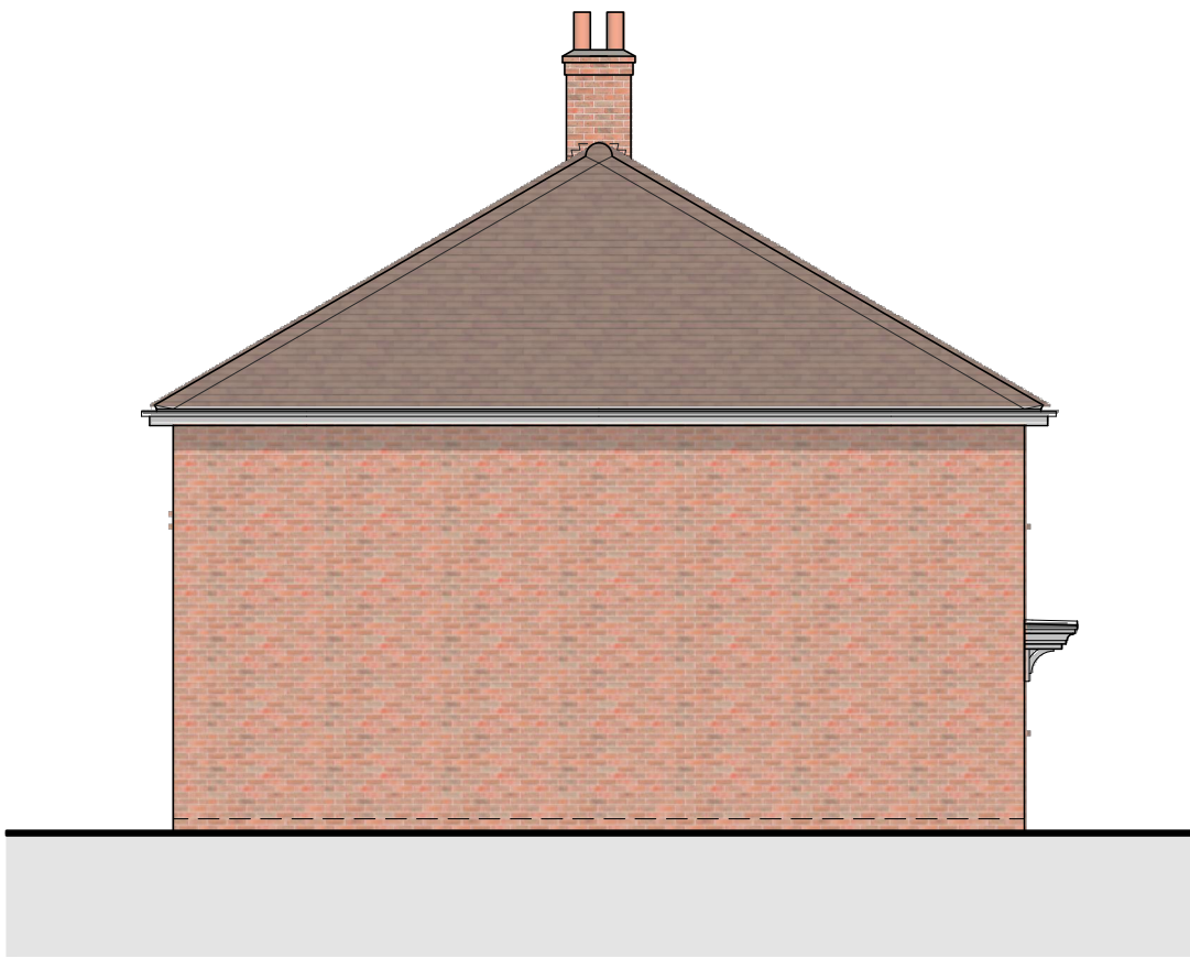
SIDE elevation
