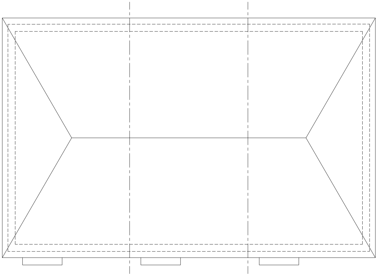
ROOF plan
