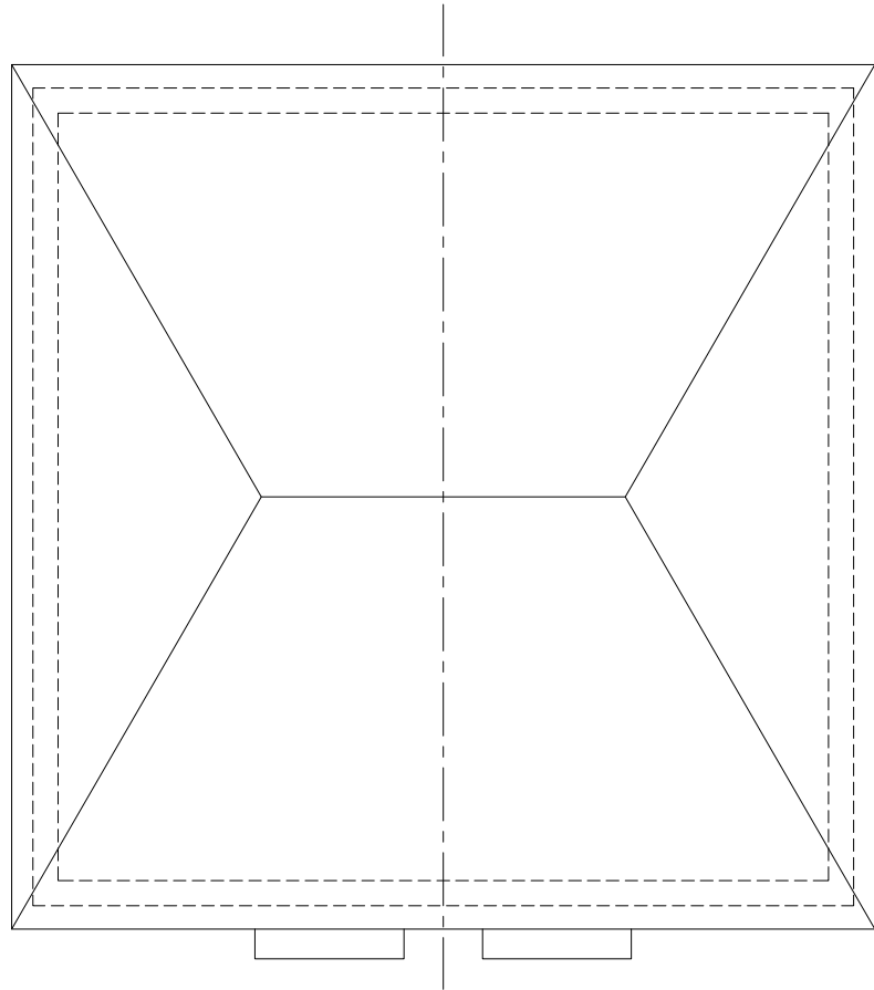
ROOF plan
