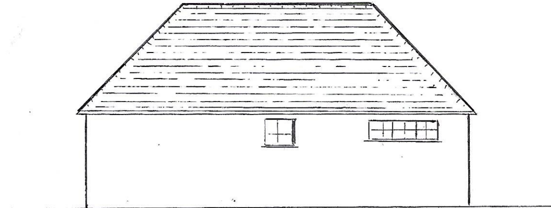
Existing, West (Rear) Elevation Scale 1:100
