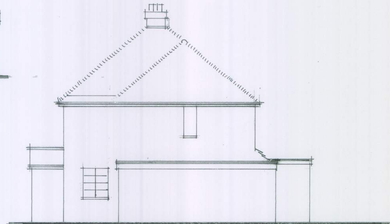
EXISTING NORTH ELEVATION 1-100
