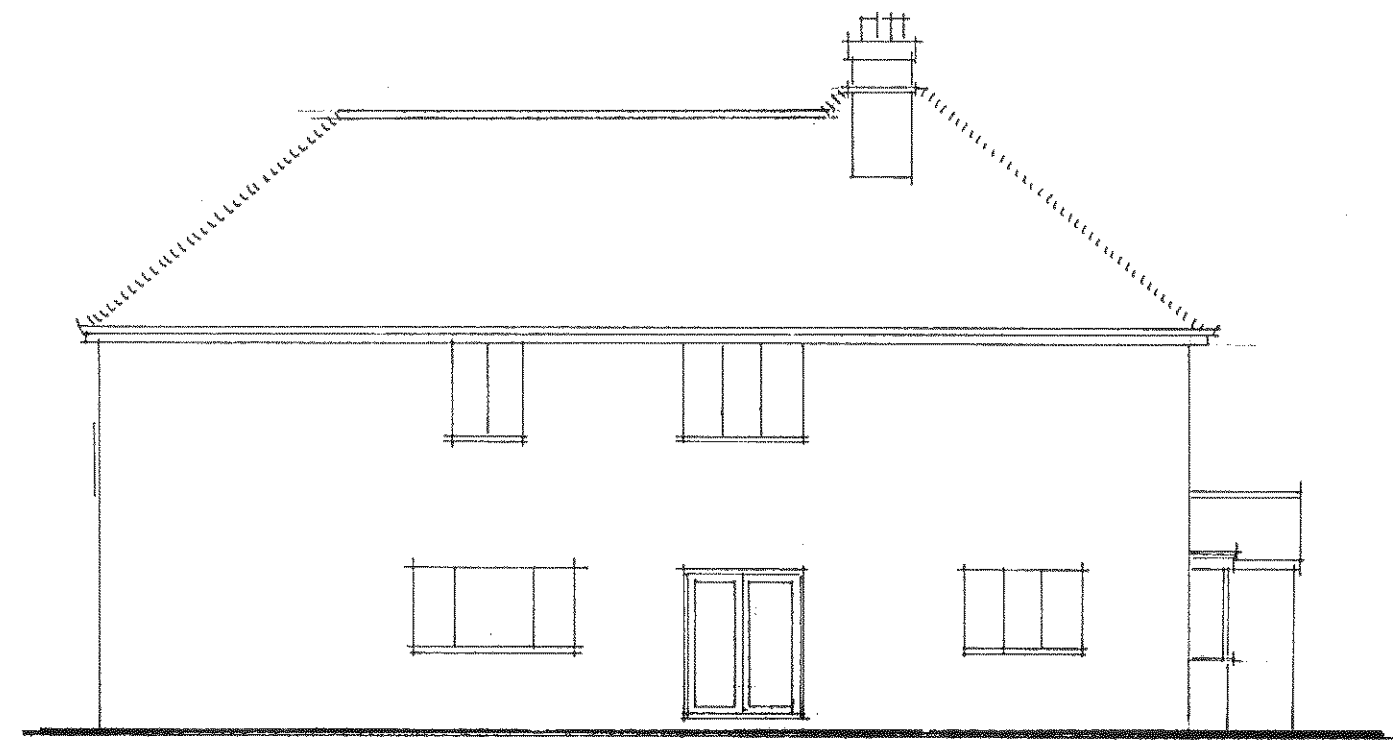
PROPOSED SOUTH ELEVATION 1-100 PROPOSED ELEVATIONS
