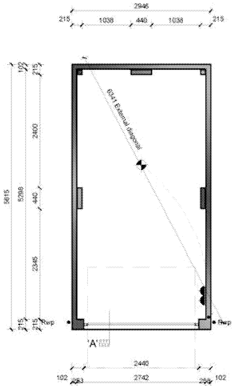
Floor Plan
